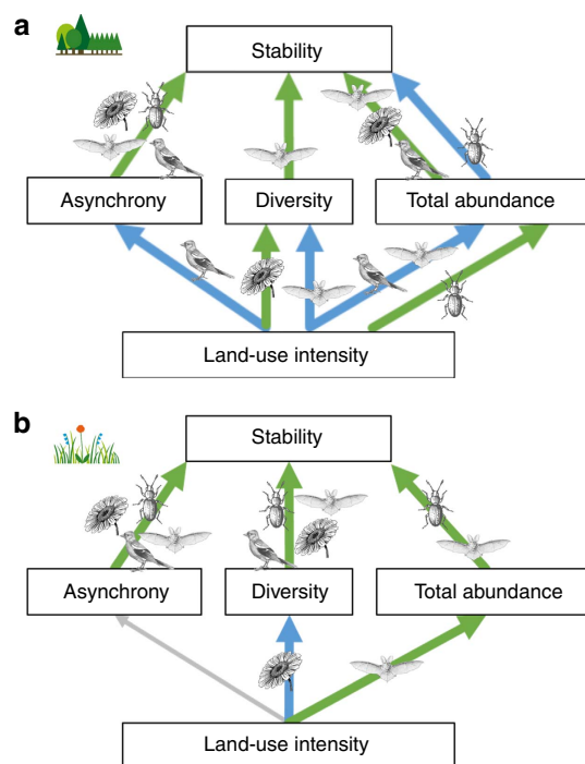
Figure 3 | Indirect effects of land-use intensity on community stability.
