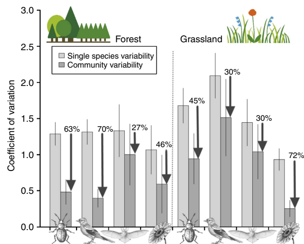
Figure 1 | Stabilization gain by communities compared with single species. Communities had a lower inter-annual variability (coefficient of variation, CV_{tot} ) in total abundance than single species ( CV_{sp} ). The figure shows strong decreases in CV_{tot} —and thus increased stability (arrows)—compared with the mean CV_{sp} , resulting from portfolio effects and species asynchrony. Four taxa (arthropods, birds, bats and plants) in forests and grasslands were compared. Differences in stability between forests and grasslands in interaction with taxon were highly significant, whereas the relative stability gain ( CV_{sp}/CV_{tot} ) between the two habitats was not. Each bar shows mean \pm s.d. across all plots ( N=135 – 150 plots, except forest arthropods: N=30 ).
